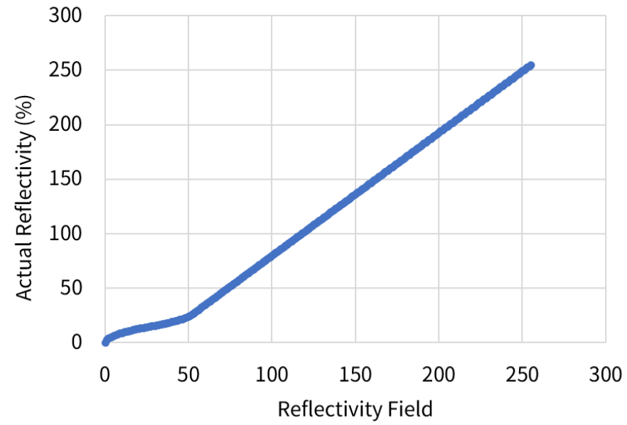
Figure 28. Nonlinear mapping 2#
